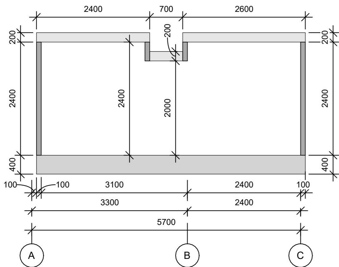
Section 2-2
