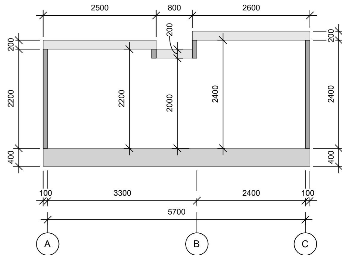
Section 3-3
